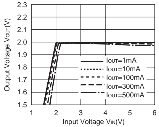
R1171x201B
