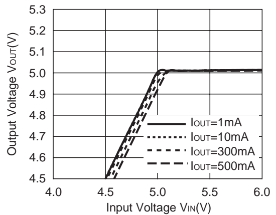
R1171x501B
