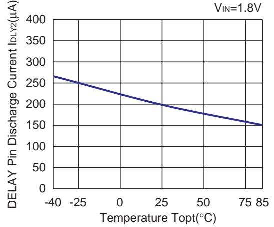
9) DELAY Pin Discharge Current vs. Temperature R1215D002x
