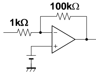
Error Amplifier
