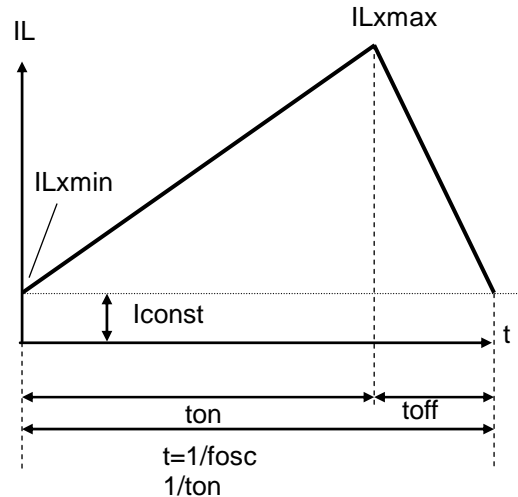
Continuous Mode
