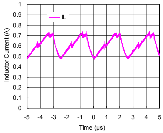
5LED(V IN =3V) R1202N723D
