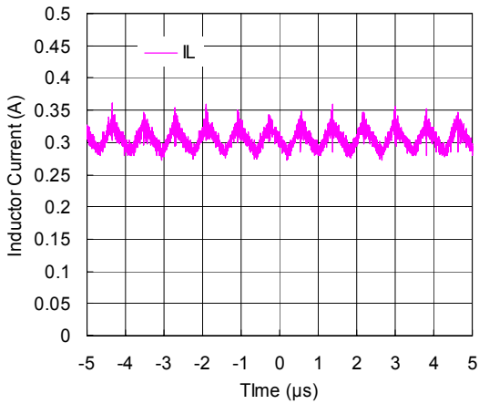
5LED(V IN =3.6V) R1202N713D
