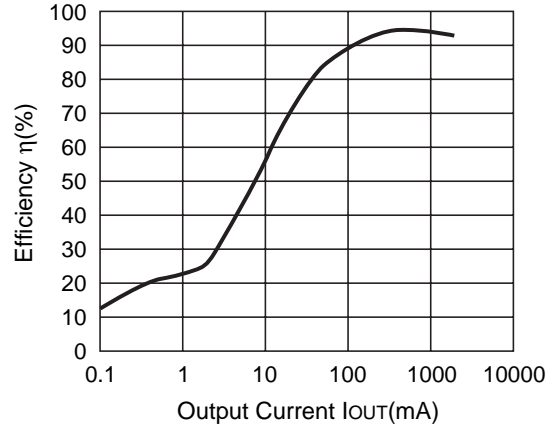
R1225N332C (V IN =4.8V) CDRH127-10μH
