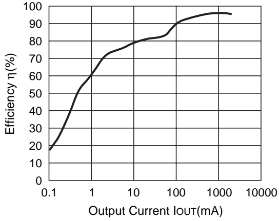
R1225N502A (V IN =6.5V) CDRH127-10μH
