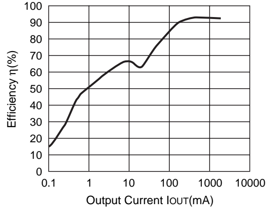
R1225N332B (V IN =4.8V) CDRH127-10μH
