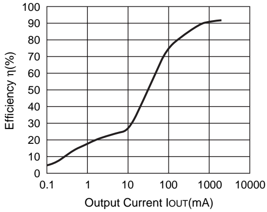
R1225N502K (V IN =15V) CDRH127-27μH
