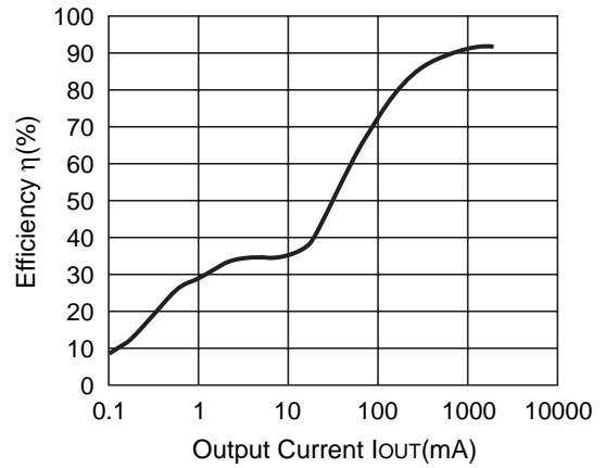
R1225N502C (V IN =12V) CDRH127-10μH
