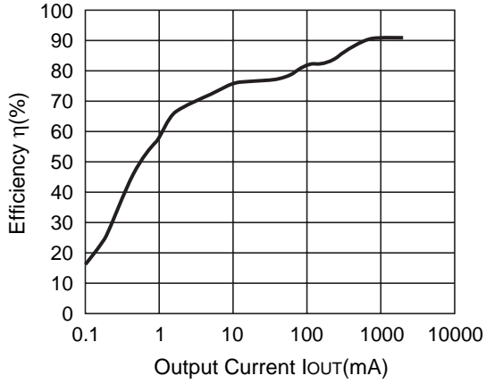
R1225N332B (V IN =7.0V) CDRH127-10μH
