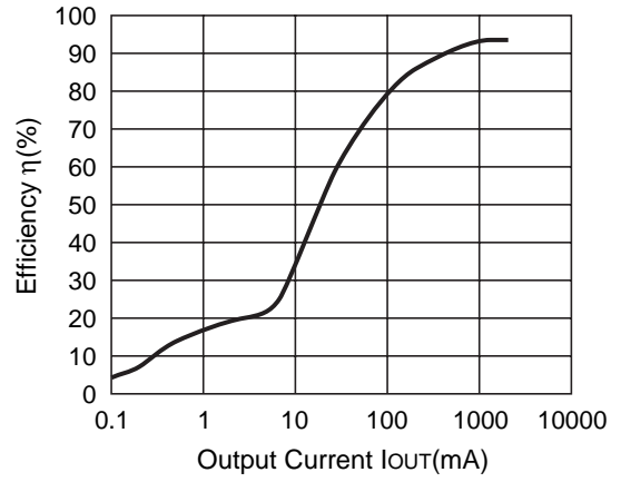
R1225N502K (V IN =12V) CDRH127-27μH
