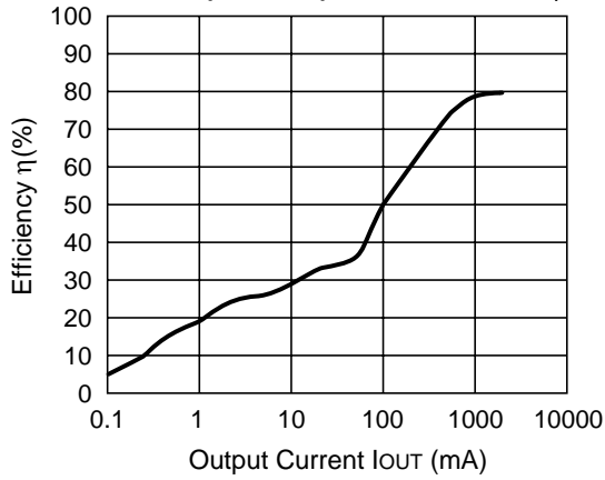
R1225N182C (V IN =12V) CDRH127-10μH
