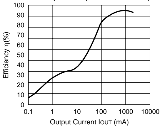
R1225N182D (V IN =5.0V) CDRH127-10μH
