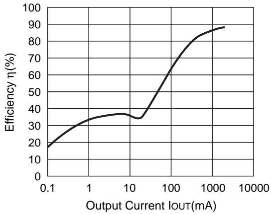
R1225N332C (V IN =12V) CDRH127-10μH
