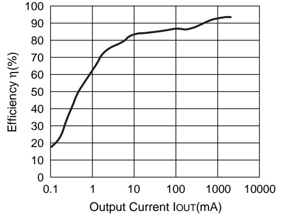
R1225N502A (V IN =10V) CDRH127-10μH
