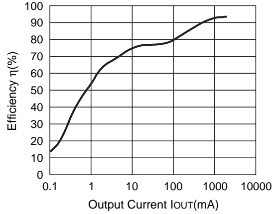
R1225N502B (V IN =10V) CDRH127-10μH
