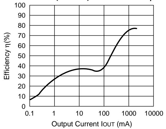
R1225N182D (V IN =12V) CDRH127-10μH
