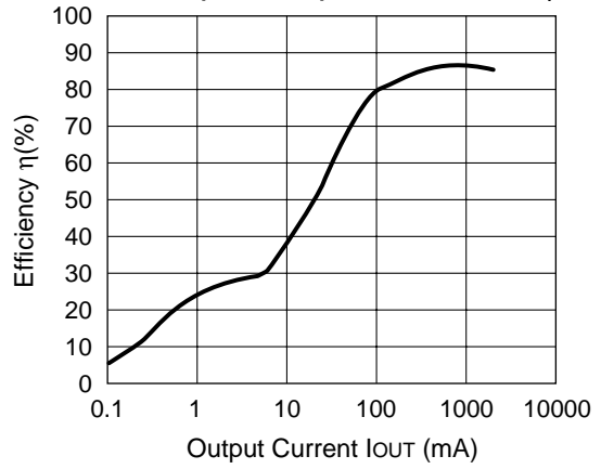
R1225N182C (V IN =5.0V) CDRH127-10μH
