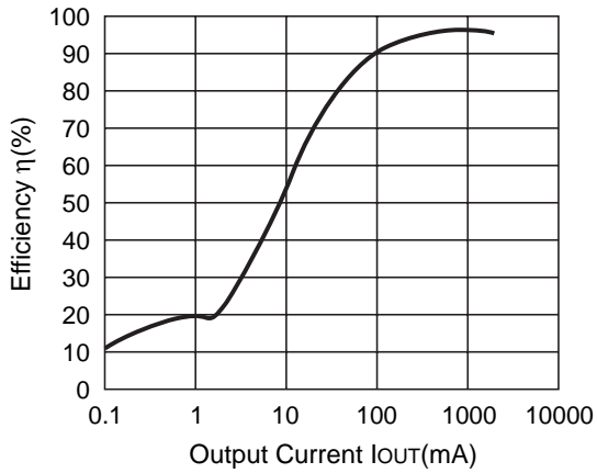
R1225N502C (V IN =6.5V) CDRH127-10μH
