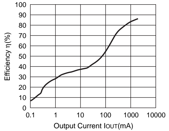
R1225N332C (V IN =15V) CDRH127-10μH
