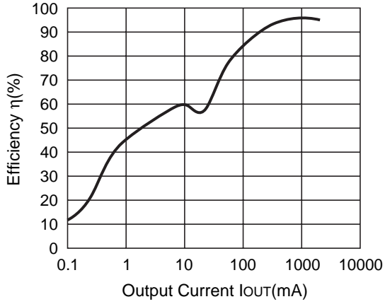
R1225N502B (V IN =6.5V) CDRH127-10μH
