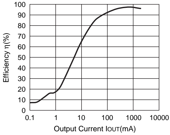
R1225N502K (V IN =6.5V) CDRH127-27μH
