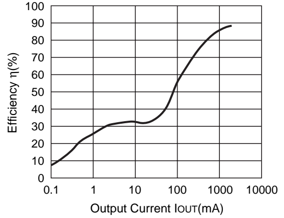
R1225N502D (V IN =15V) CDRH127-10μH
