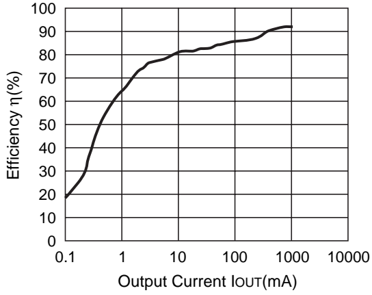
R1225N332A (V IN =7.0V) CDRH127-10μH
