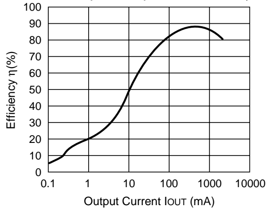
R1225N182D (V IN =3.3V) CDRH127-10μH
