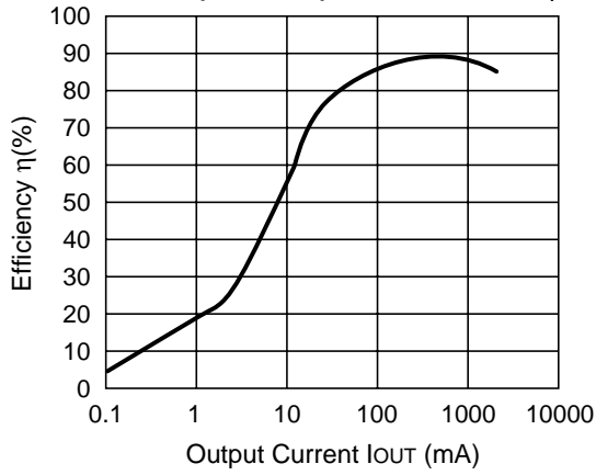
R1225N182C (V IN =3.3V) CDRH127-10μH
