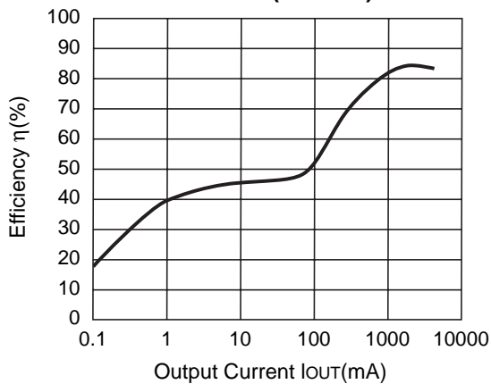
R1224N332G ( V_{IN}=16V )
